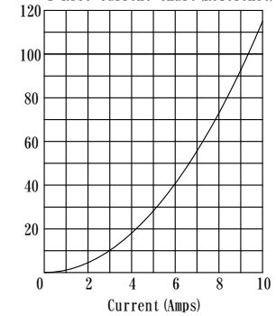
T-Rise Current Chart (Reference)
