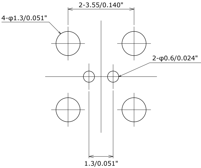
PC Board Layout (Top View)
