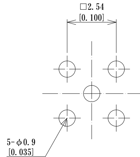
PCB Mounting Layout
