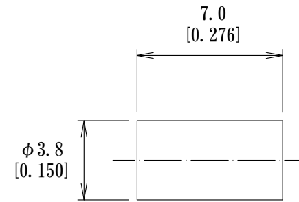
Crimp Ring
