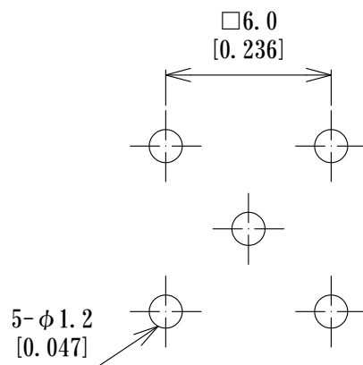
PCB Mounting Layout
