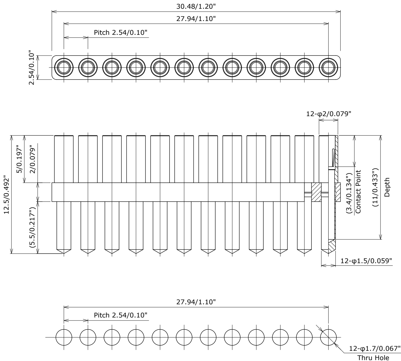
PC Board Layout (Top View)
