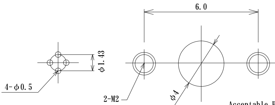
PCB dimension
