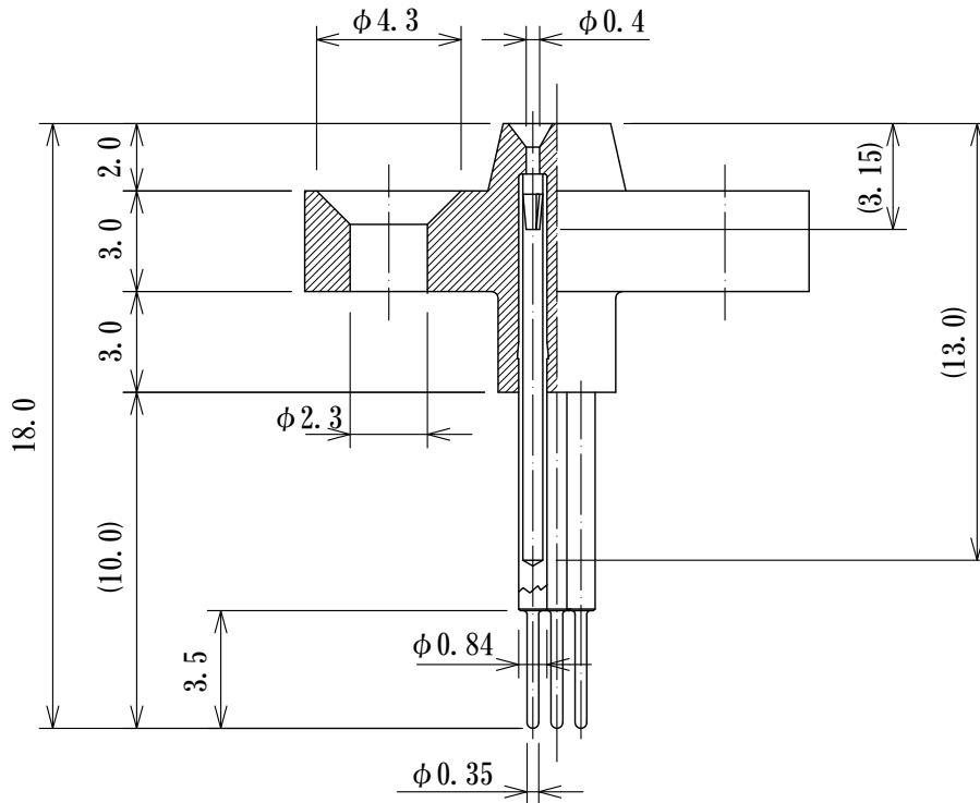
PCB dimension
