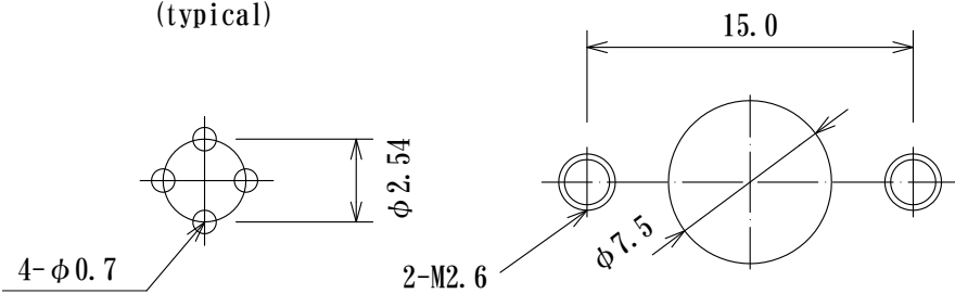
Mounting Dimension
