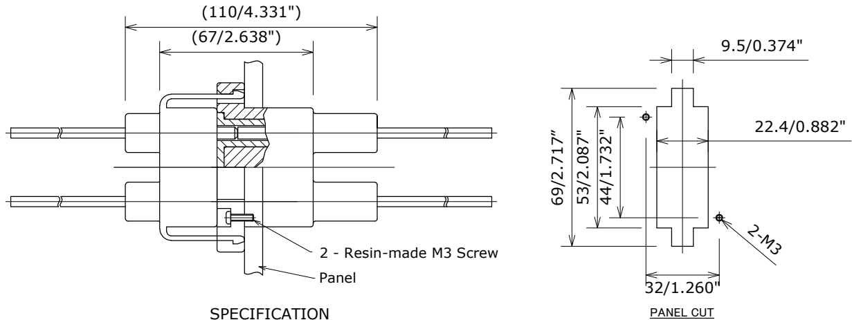
Example of Mating (2) When Using a Panel
